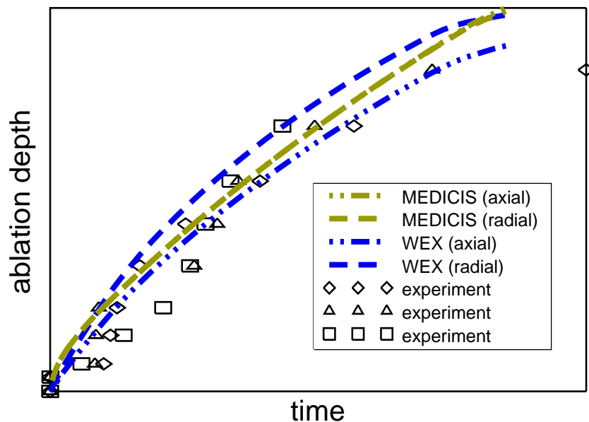
Figure 11: Ablation depths calculated by WEX and MEDICIS for CCI 2 in a blind calculation
