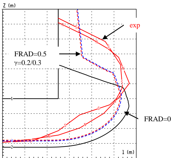
CCI2 T_{solidif}(\gamma=0.2, 0.3) , FRAD=0, 0.5 Cavity boundaries, without/with upwards radiation contributing to ablation
