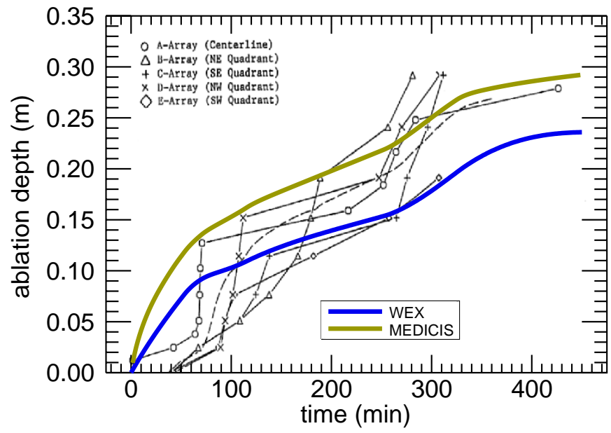
Figure 9: Ablation depths calculated by WEX and MEDICIS for MACE-M3b.
