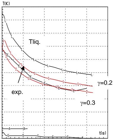
CCI2 test: temperature evolution Corium temperature, T_{sol} , T_{liq} , \gamma=0.2, 0.3 , FRAD=0.5
