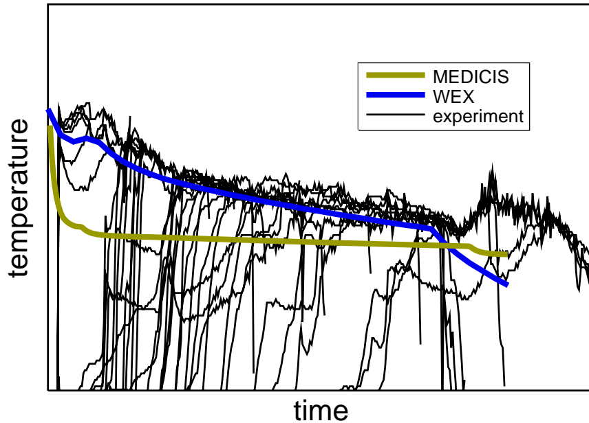
Figure 10: Melt temperature calculated by WEX and MEDICIS for CCI 2 in a blind calculation
