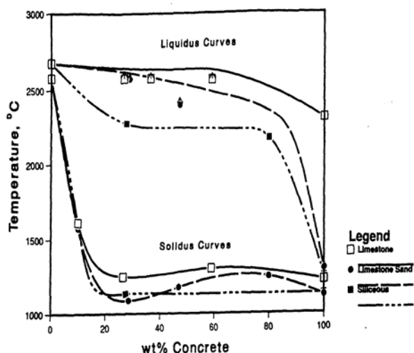
Figure 2: Liquids- and solidus temperatures for quasi-binary core-concrete mixtures
