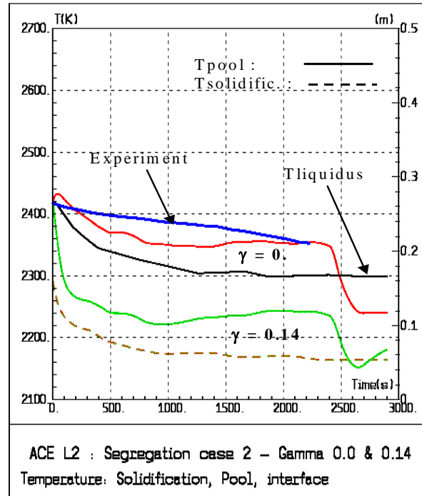
Figure 5: Temperature evolution in L2 with refractory material segregation in crusts
