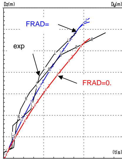
CCI2: T_{solidif}(\gamma) , \gamma=0.2 , h_{conv} BALI Cavity Boundaries FRAD=0, 0.5
