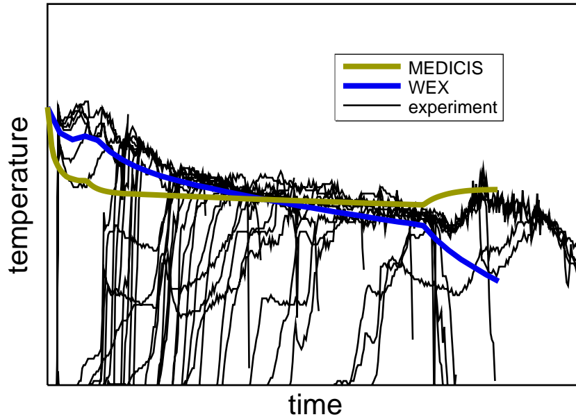
Figure 12: Melt temperature calculated by WEX and MEDICIS for CCI 2 after adapting heat transfer correlations in MEDICIS
