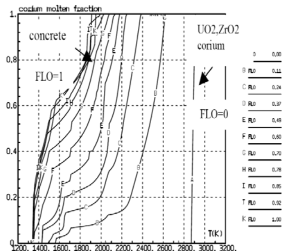
Figure 3: Molten fraction versus temperature T and light oxide fraction (FLO) evaluated by the code GEMIN2 for MEDICIS
