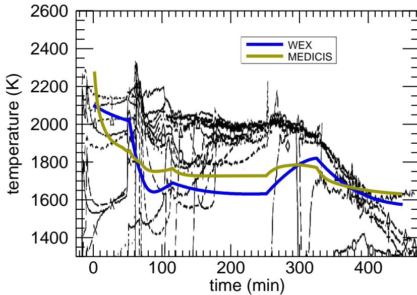
Figure 8: Melt temperature calculated by WEX and MEDICIS for MACE-M3b.
