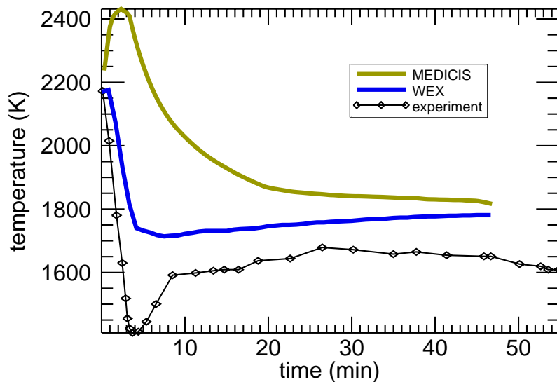
Figure 6: Melt temperature calculated by WEX and MEDICIS for BETA V5.2
