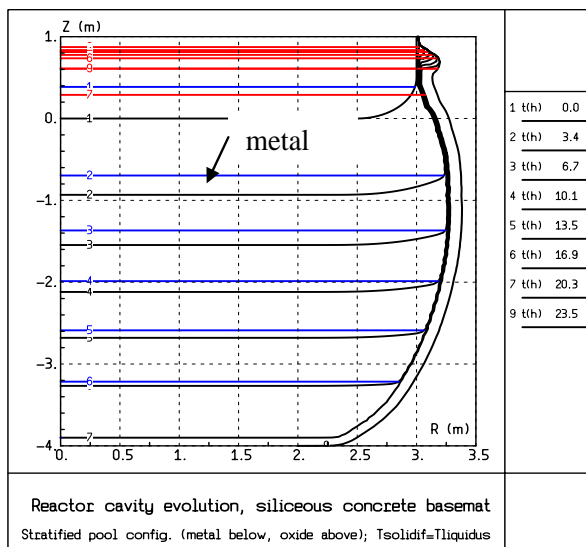
Figure 18: Erosion of reactor cavity with stratified configuration; melt-through at 23.5 h (stratTliq)
