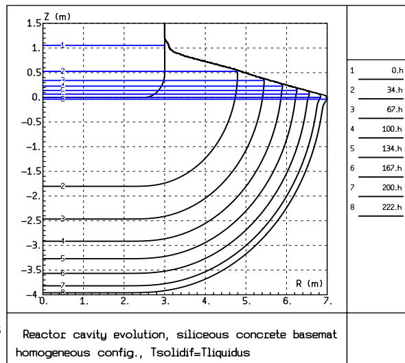
Figure 17: Cavity erosion with homogeneous configuration; melt-through at 222 h (hgTliq)
