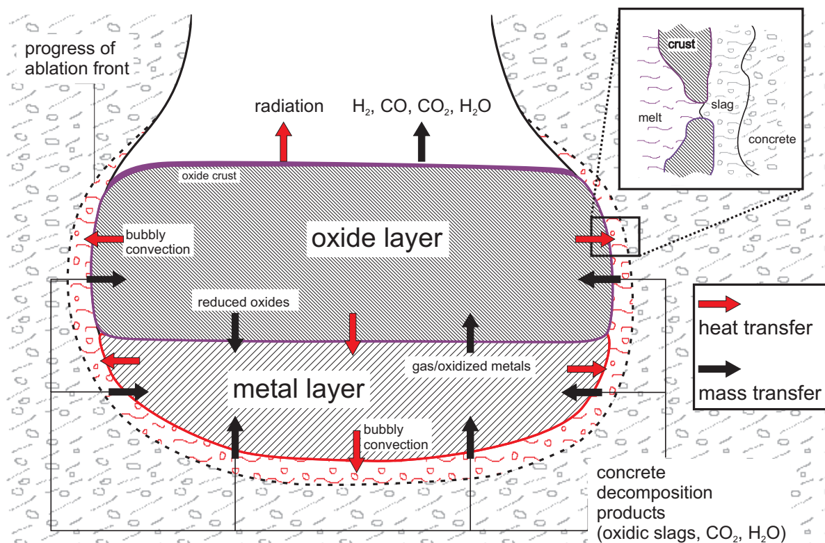
Figure 1: Basic sketch of a stratified two-layer configuration of the molten pool (metal below oxide) and the relevant heat and mass transfer pathways to be regarded for the simulation of MCCI phenomena
