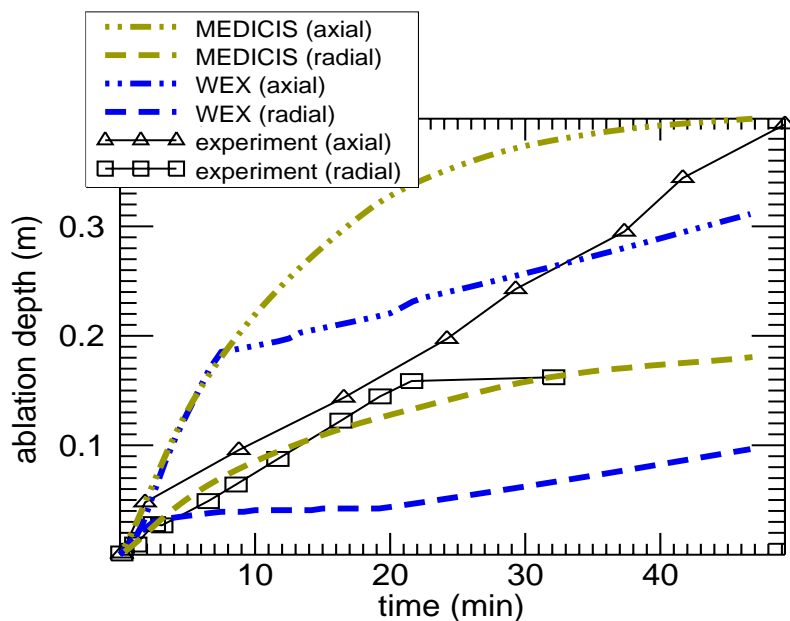
Figure 7: Ablation depths calculated by WEX and MEDICIS for BETA 5.2
