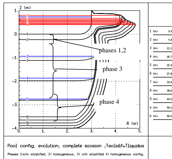
Figure 19: Case with pool configuration evolution in 4 phases until basemat melt-through at 50.5 h
