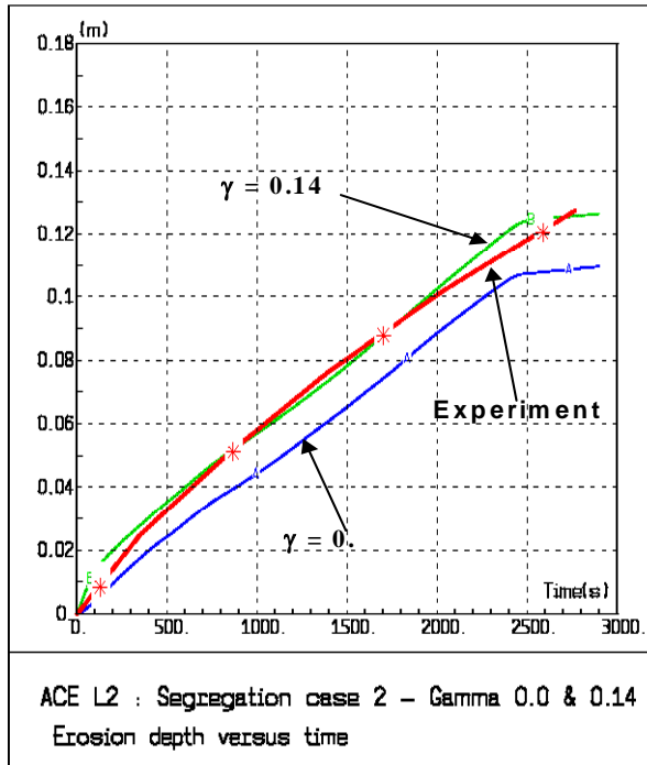
Figure 4: Concrete ablation kinetics in L2 with refractory material segregation in crusts
