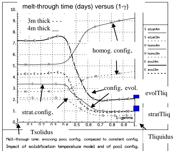
Figure 16: Melt-through time versus freezing temperature and configuration evolution
